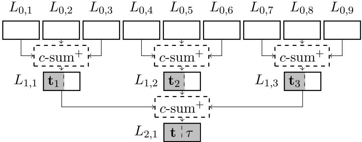
Figure 2: An illustration of the c -sum + BKW for c = 3 , where \mathbf{t} = \mathbf{t}_1 + \mathbf{t}_2 + \mathbf{t}_3
